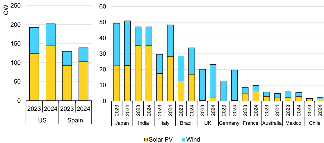
Solar PV and wind projects in late-stage development by market, 2023 and 2024
